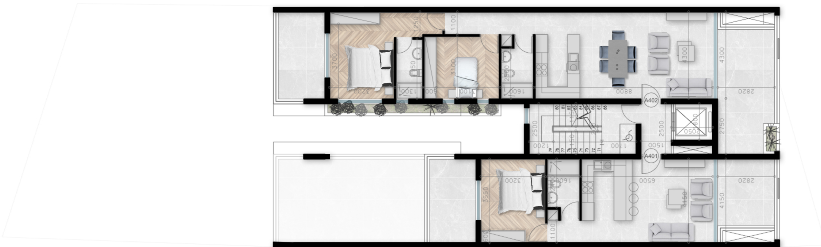
fourth floor
